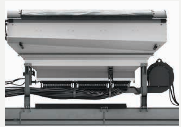
The optional dry fertilizer system features 170 cu. ft. of capacity and is conveniently located on the planter tongue.
